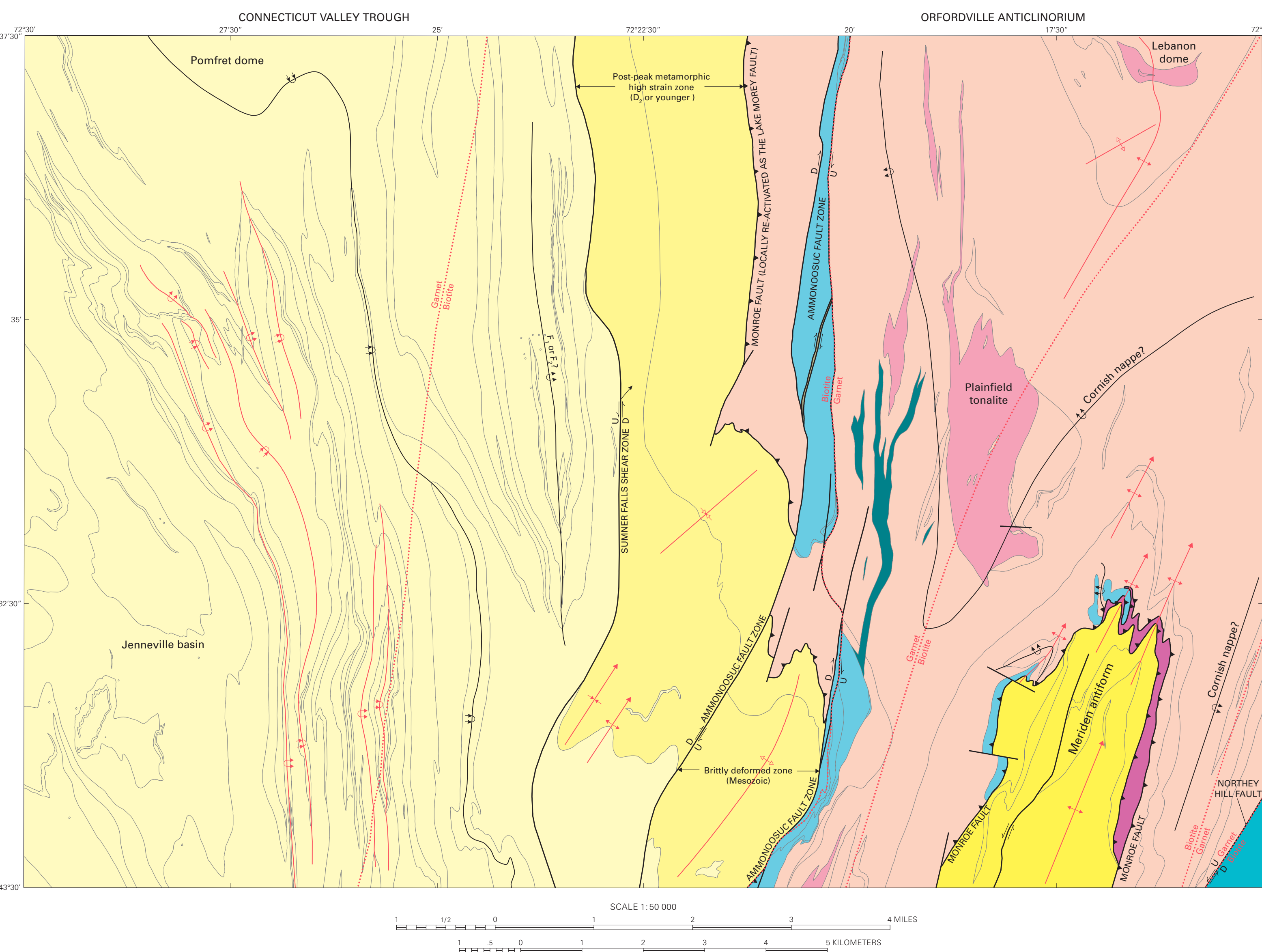
Figure 1.—Tectonic map showing major structural features of the Hartland and North Hartland quadrangles.
