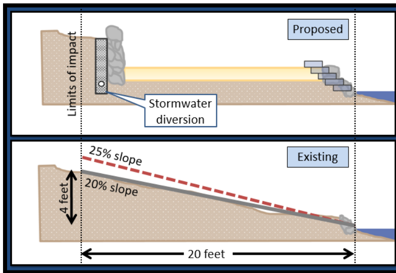
Figure 2 - Cross-section of a proposed perched beach. Note that the slope calculation includes the location of the proposed swale and steps and that the beach is located landward and above the hardened shoreline.
