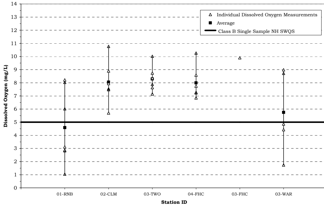
Figure 2. Dissolved Oxygen Statistics for the Lower Cochecho River Watershed - Rollinsford May 19 - September 18, 2007, NHDES VRAP
