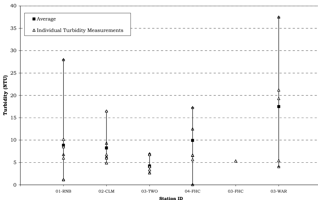
Figure 4. Turbidity Statistics for the Lower Cocheco River Watershed - Rollinsford May 19 - September 18, 2007, NHDES VRAP
