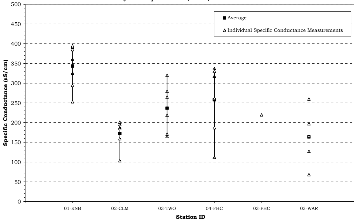
Figure 5. Specific Conductance Statistics for the Lower Cocheco River Watershed - Rollinsford May 19 - September 18, 2007, NHDES VRAP
