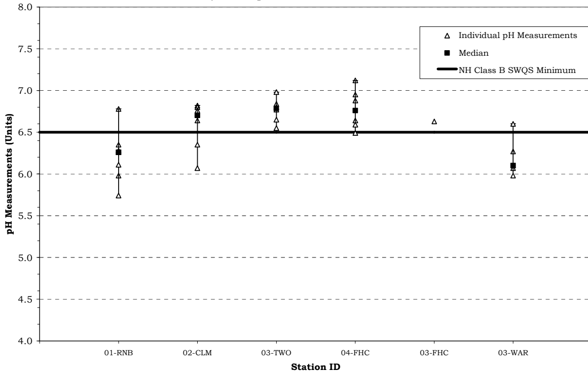
Figure 3. pH Statistics for the Lower Cocheco River Watershed - Rollinsford May 19 - September 18, 2007, NHDES VRAP
