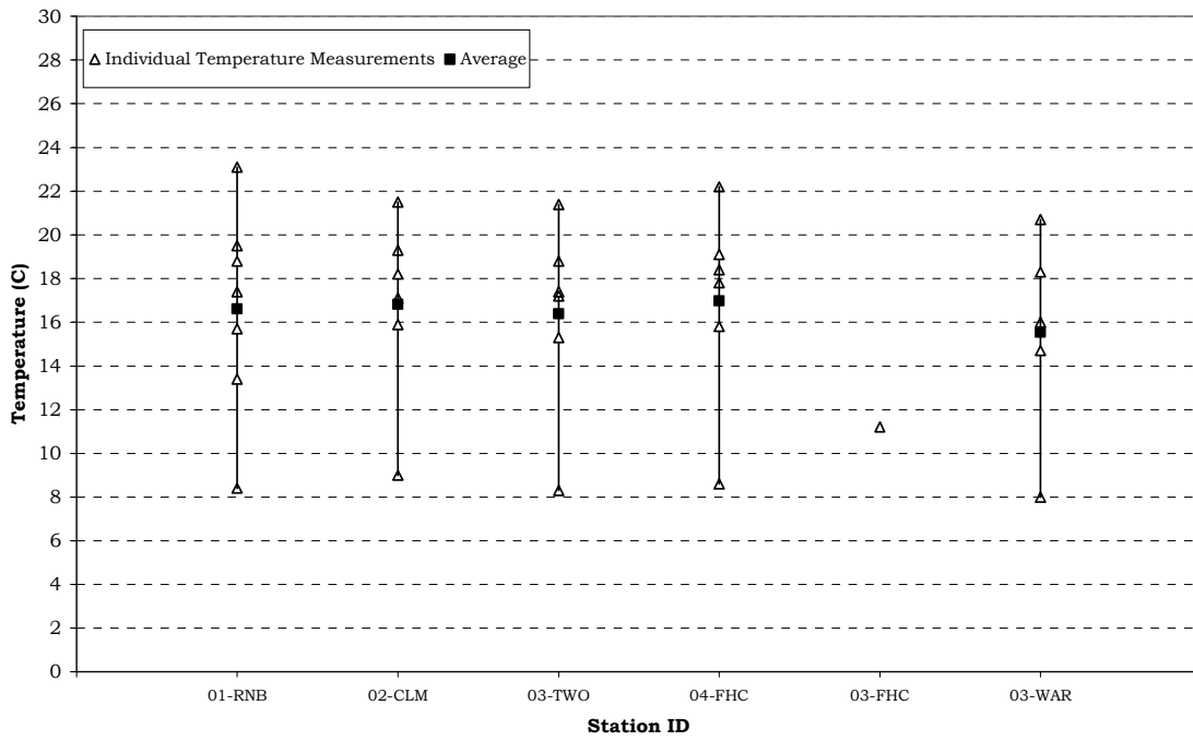
Figure 6. Water Temperature Statistics for the Lower Cocheco River Watershed - Rollinsford May 19 - September 18, 2007, NHDES VRAP
