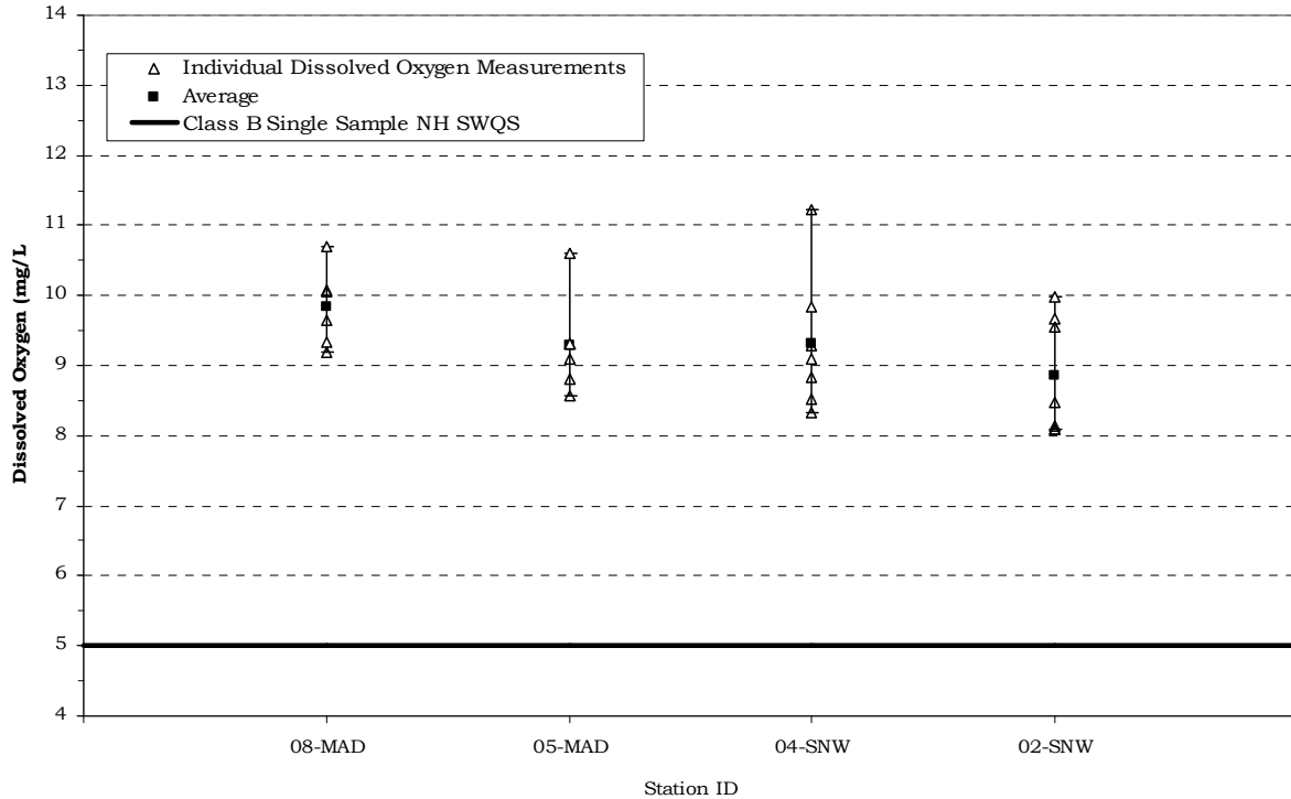
Figure 2. Dissolved Oxygen Concentration Statistics for Mad River & Snows Brook May 10 - October 16, 2008, NHDES VRAP
