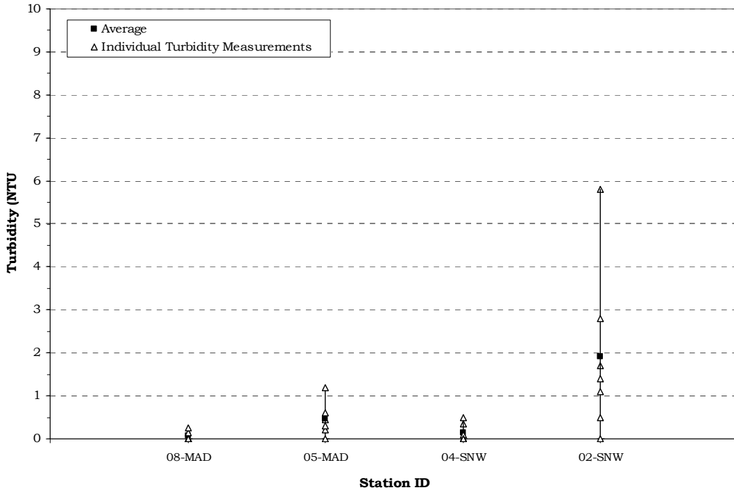
Figure 4. Turbidity Statistics for Mad River & Snows Brook May 10 - October 16, 2008, NHDES VRAP
