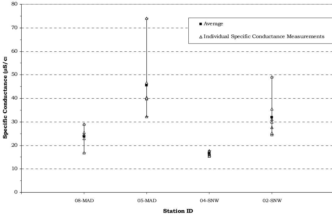
Figure 5. Specific Conductance Statistics for Mad River & Snows Brook May 10 - October 16, 2008, NHDES VRAP
