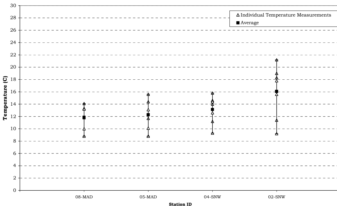
Figure 6. Water Temperature Statistics for Mad River & Snows Brook May 10 - October 16, 2008, NHDES VRAP
