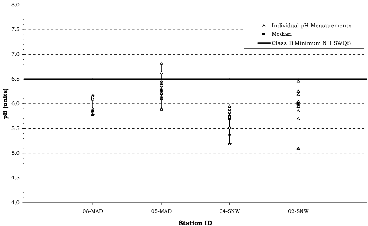
Figure 2. pH Statistics for Mad River & Snows Brook May 12 - October 27, 2010, NHDES VRAP
