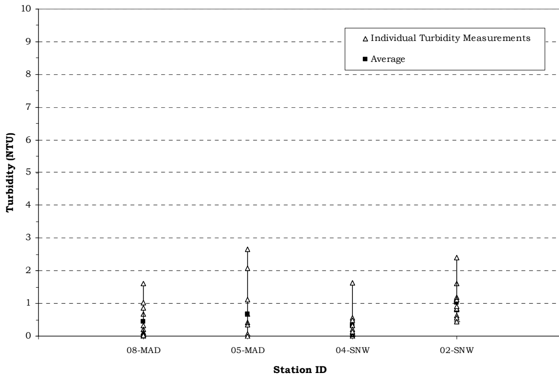
Figure 3. Turbidity Statistics for Mad River & Snows Brook May 12 - October 27, 2010, NHDES VRAP
