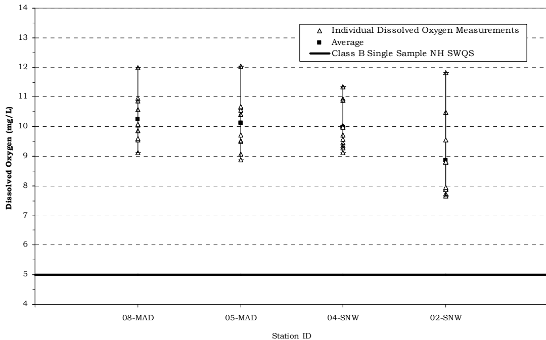
Figure 1. Dissolved Oxygen Concentration Statistics for Mad River & Snows Brook May 12 - October 27, 2010, NHDES VRAP
