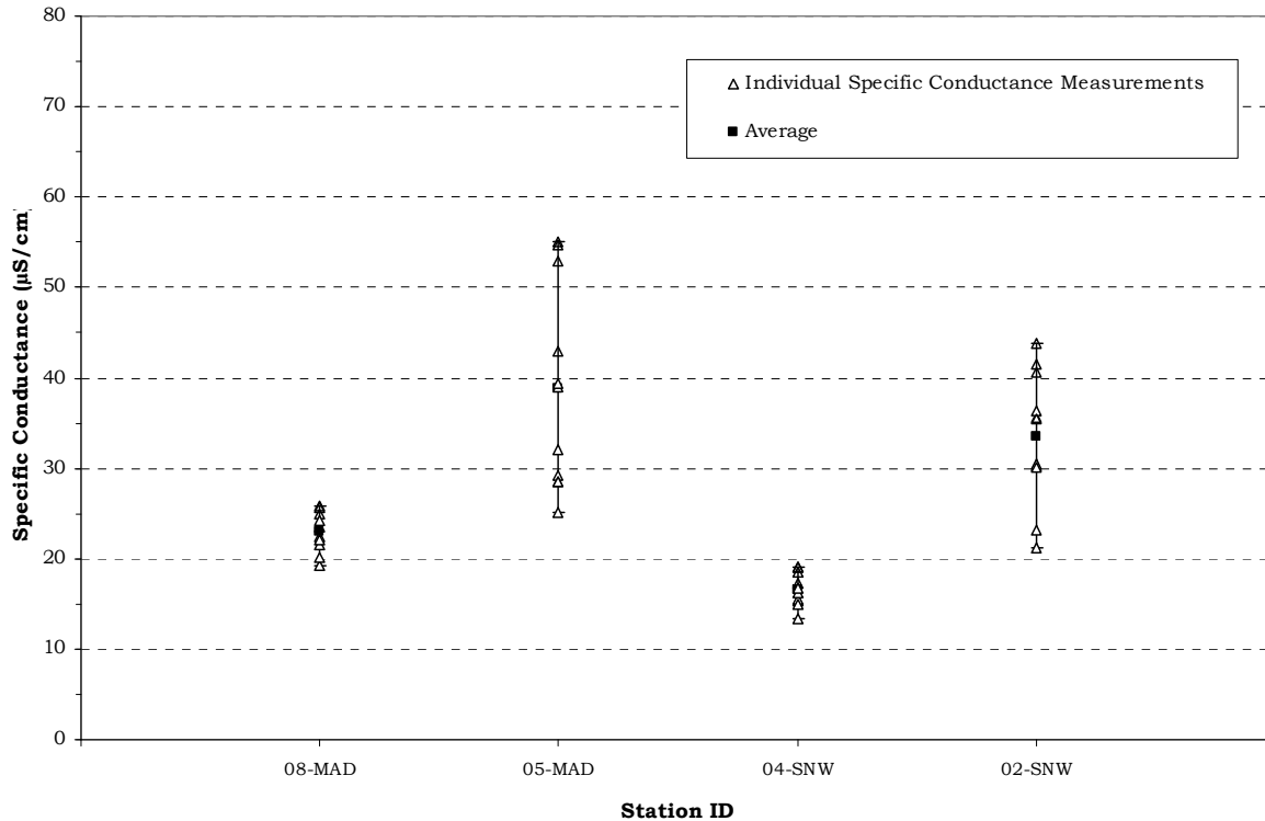
Figure 4. Specific Conductance Statistics for Mad River & Snows Brook May 12 - October 27, 2010, NHDES VRAP
