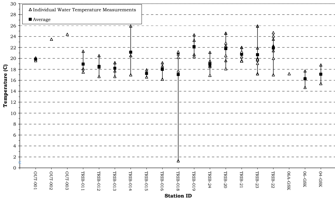
Figure 5. Water Temperature Statistics for the Paugus Bay Tributaries May 29 - August 20, 2008, NHDES VRAP
