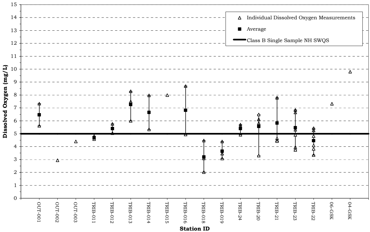
Figure 1. Dissolved Oxygen Statistics for the Paugus Bay Tributaries May 29 - August 20, 2008, NHDES VRAP
