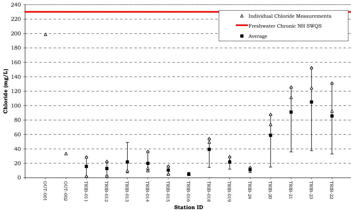
Figure 9. Chloride Statistics for the Paugus Bay Tributaries May 29, 2008 - August 20, 2008, NHDES VRAP
