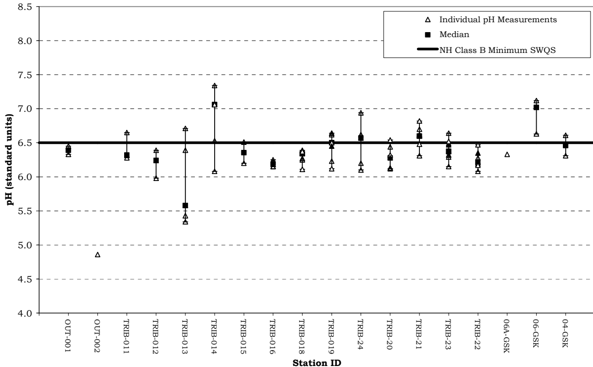
Figure 2. pH Statistics for the Paugus Bay Tributaries May 29 - August 20, 2008, NHDES VRAP
