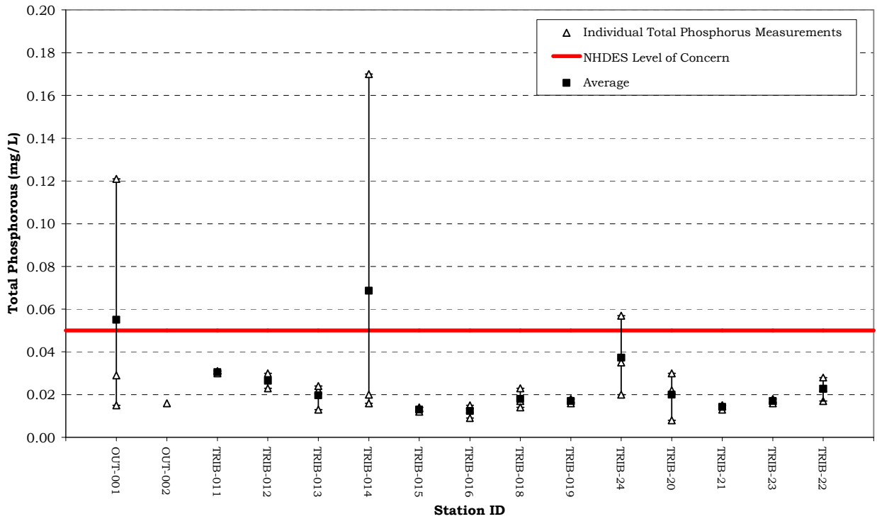
Figure 6. Total Phosphorus Statistics for the Paugus Bay Tributaries May 29 - August 20, 2008, NHDES VRAP
