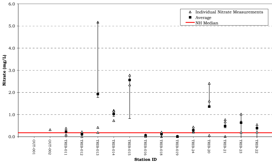
Figure 7. Nitrate Statistics for the Paugus Bay Tributaries May 29 - August 20, 2008, NHDES VRAP
