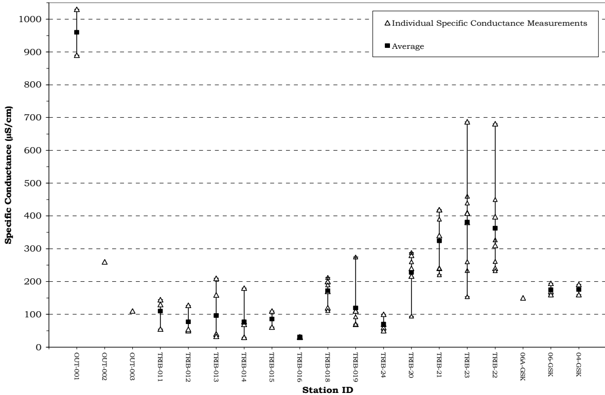
Figure 4. Specific Conductance Statistics for the Paugus Bay Tributaries May 29 - August 20, 2008, NHDES VRAP
