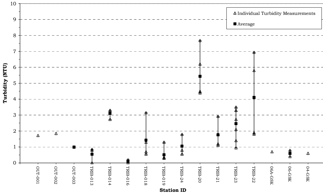
Figure 3. Turbidity Statistics for the Paugus Bay Tributaries May 29 - August 20, 2008, NHDES VRAP
